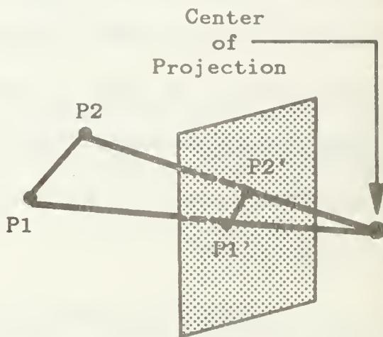
Perspective Projection
